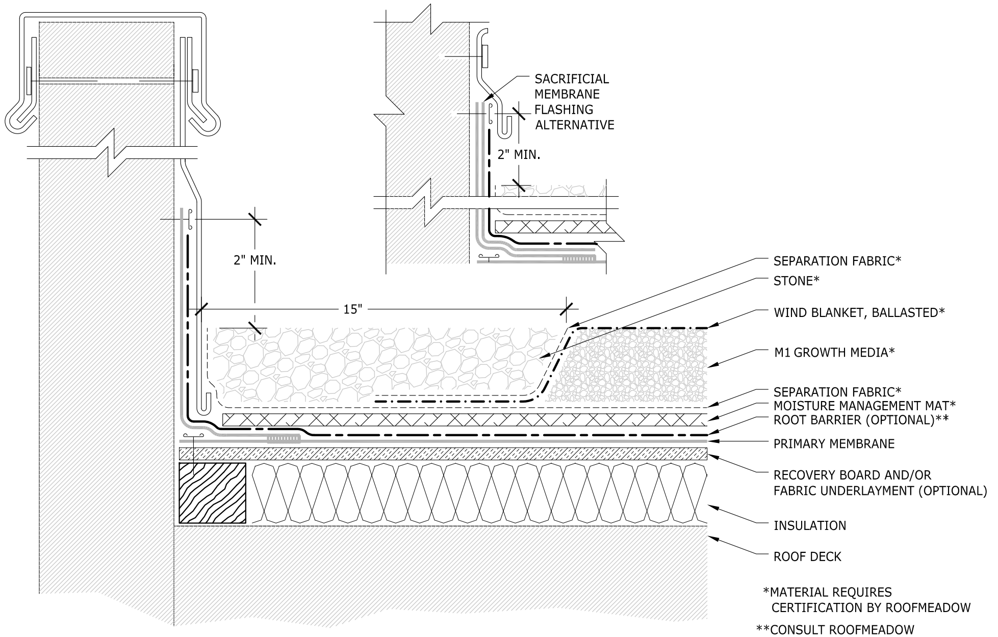
I - SINGLE MEDIA WITH MAT CONVENTIONAL CONFIG. WITH INSULATION - AT PARAPET WITH STONE BORDER
