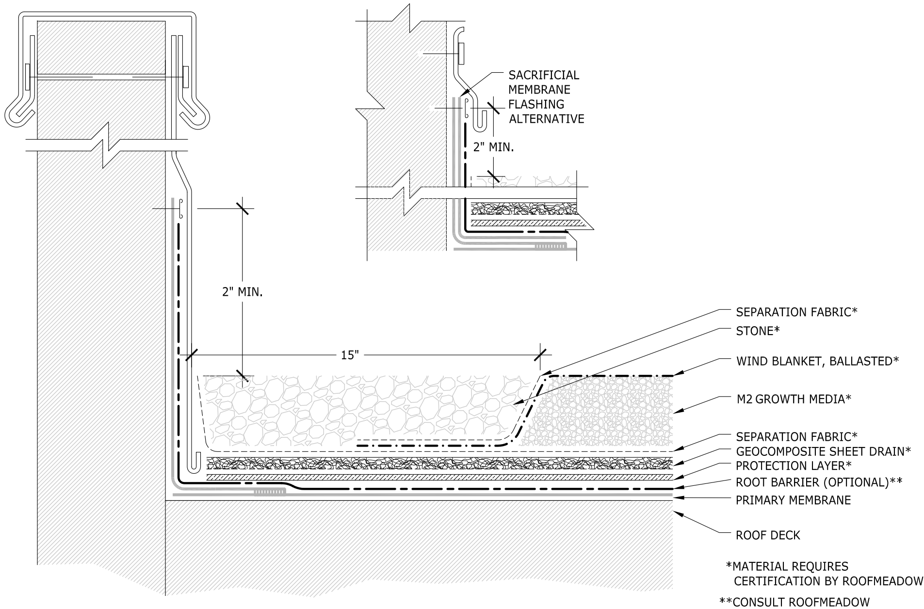
I - SINGLE MEDIA WITH MAT CONVENTIONAL CONFIG WITHOUT INSULATION - AT PARAPET WITH STONE BORDER
