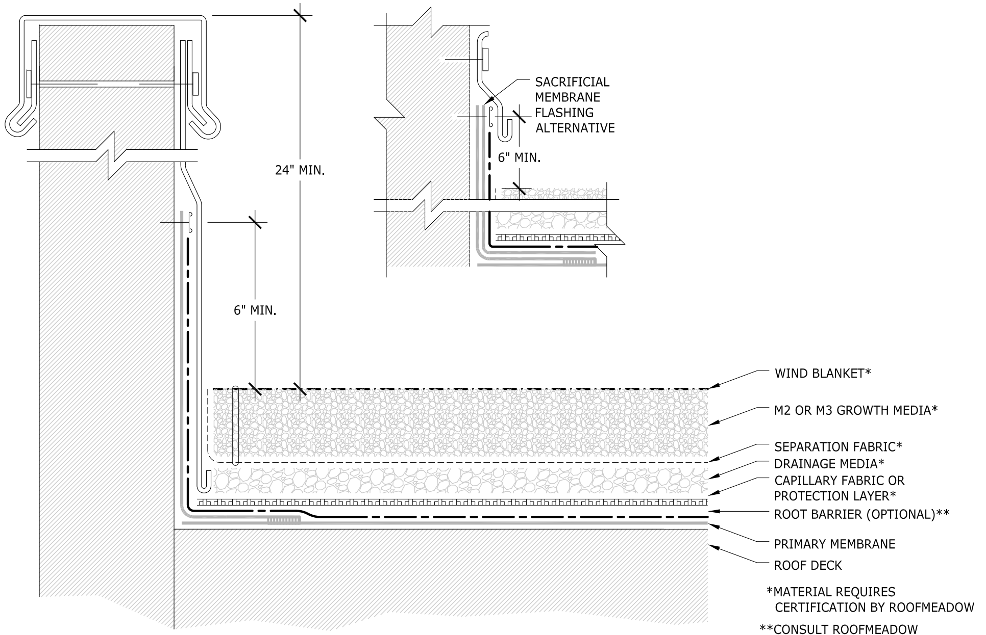
III - DUAL MEDIA CONVENTIONAL CONFIG. WITHOUT INSULATION - AT PARAPET N.T.S.
