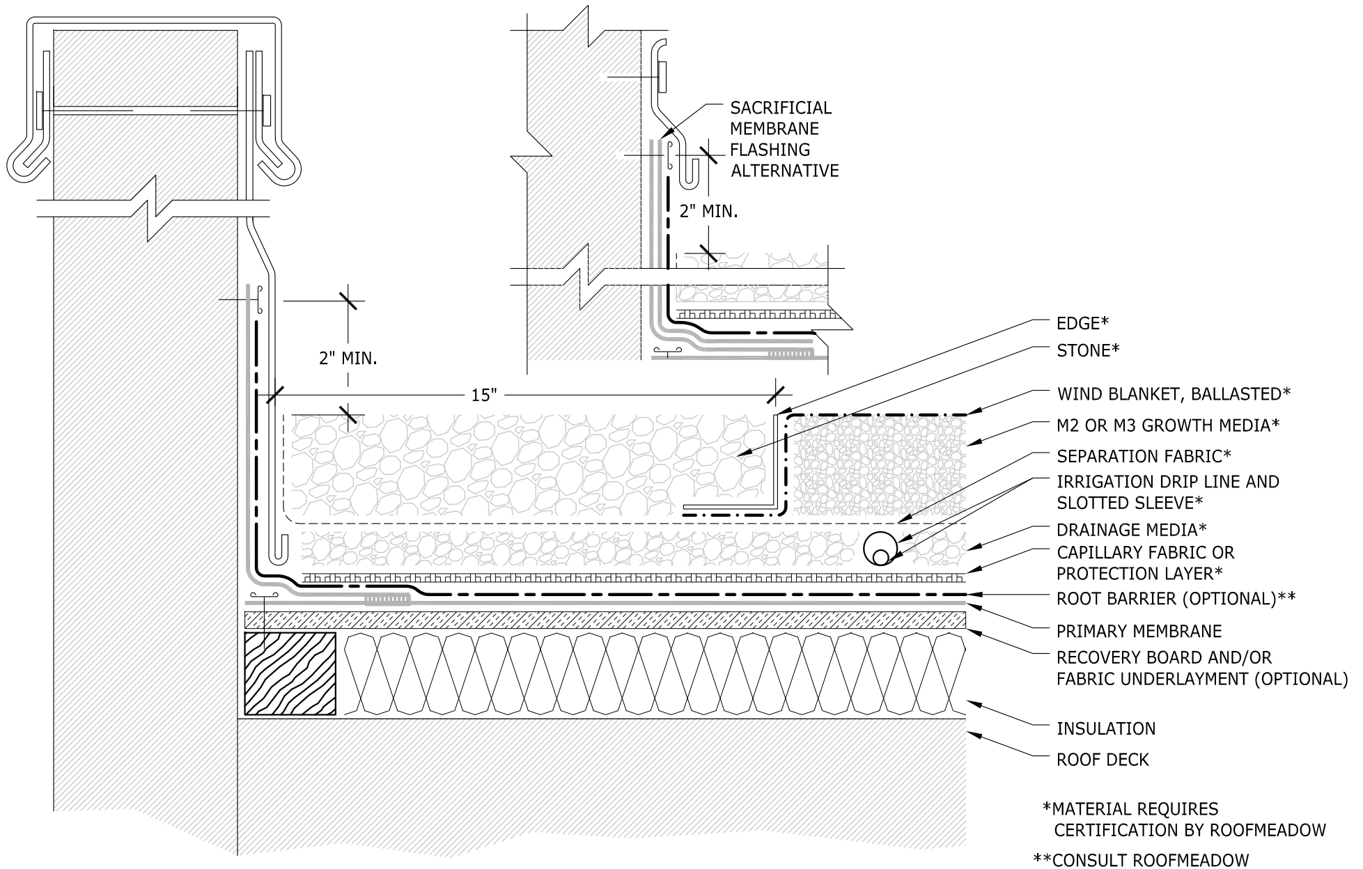
III - DUAL MEDIA CONVENTIONAL CONFIG. WITH INSULATION - AT PARAPET WITH STONE BORDER N.T.S.
