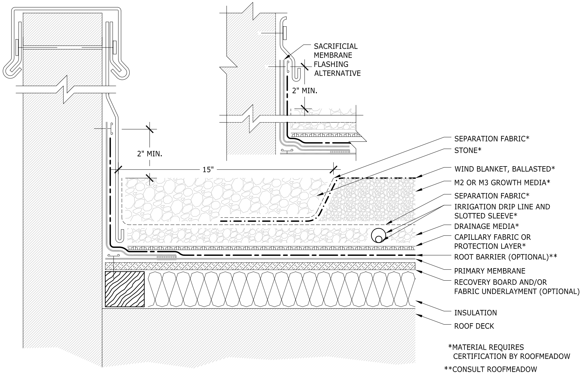
III - DUAL MEDIA CONVENTIONAL CONFIG. - AT PARAPET WITH INSULATION AND STONE BORDER N.T.S.
