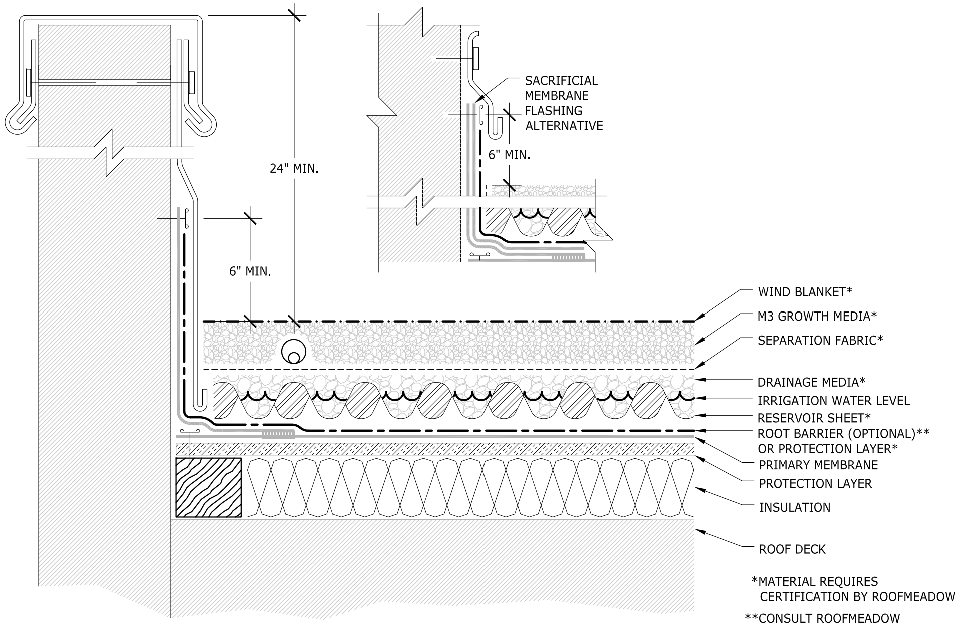
V - DUAL MEDIA WITH RESERVOIR SHEET CONVENTIONAL CONFIG. WITH INSULATION - AT PARAPET N.T.S.
