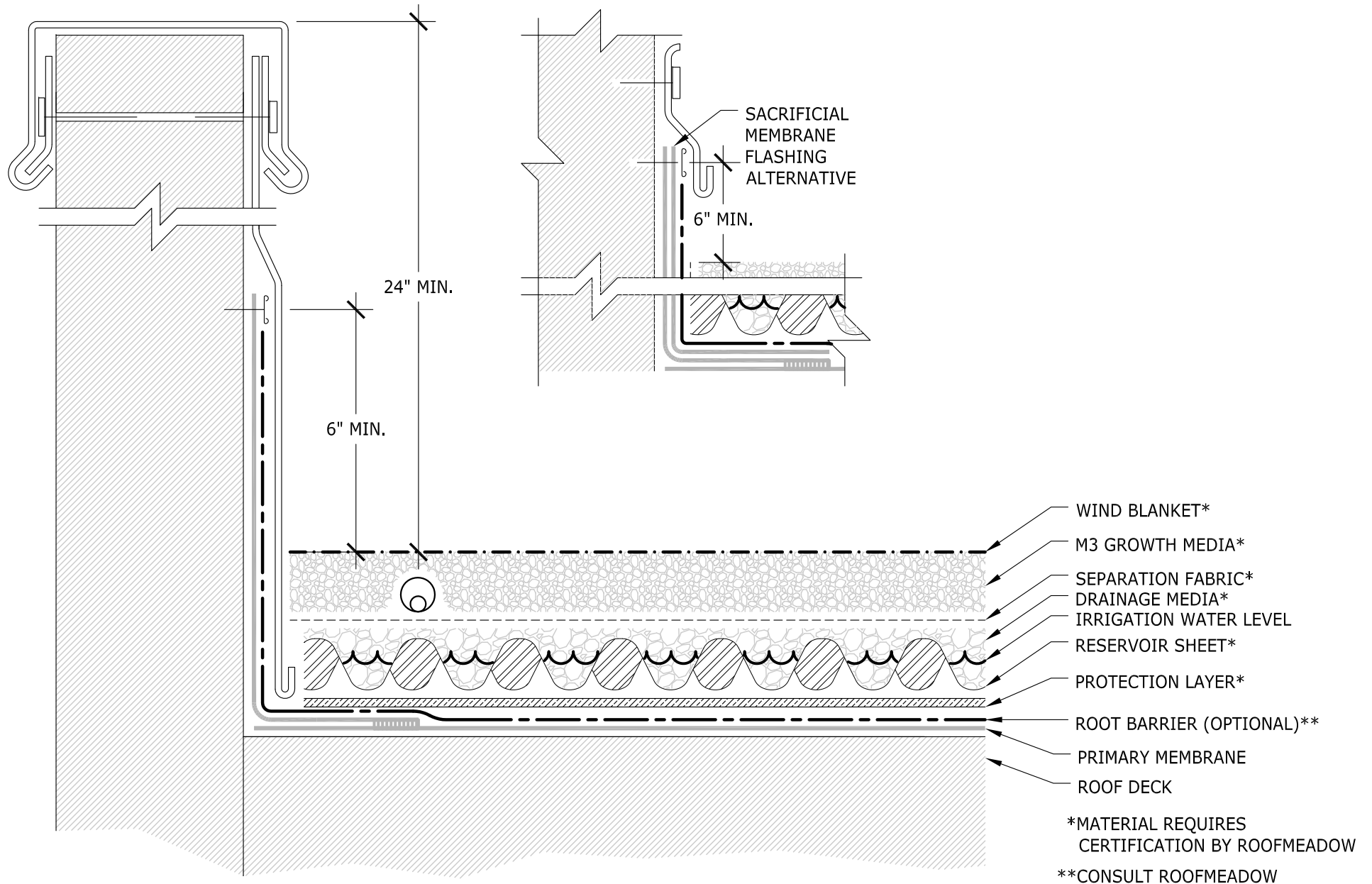
V - DUAL MEDIA WITH RESERVOIR SHEET CONVENTIONAL CONFIG. WITHOUT INSULATION - AT PARAPET N.T.S.
