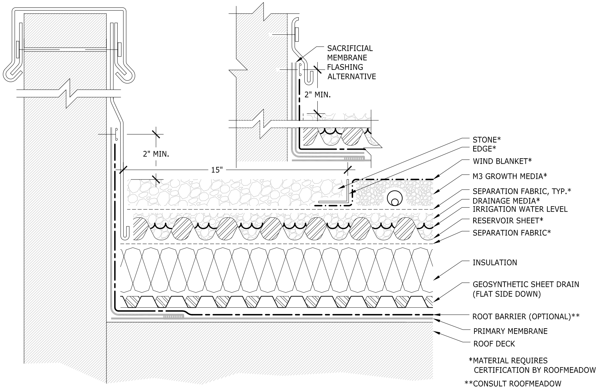
V - DUAL MEDIA WITH RESERVOIR SHEET PMR CONFIGURATION - AT PARAPET WITH STONE BORDER N.T.S.
