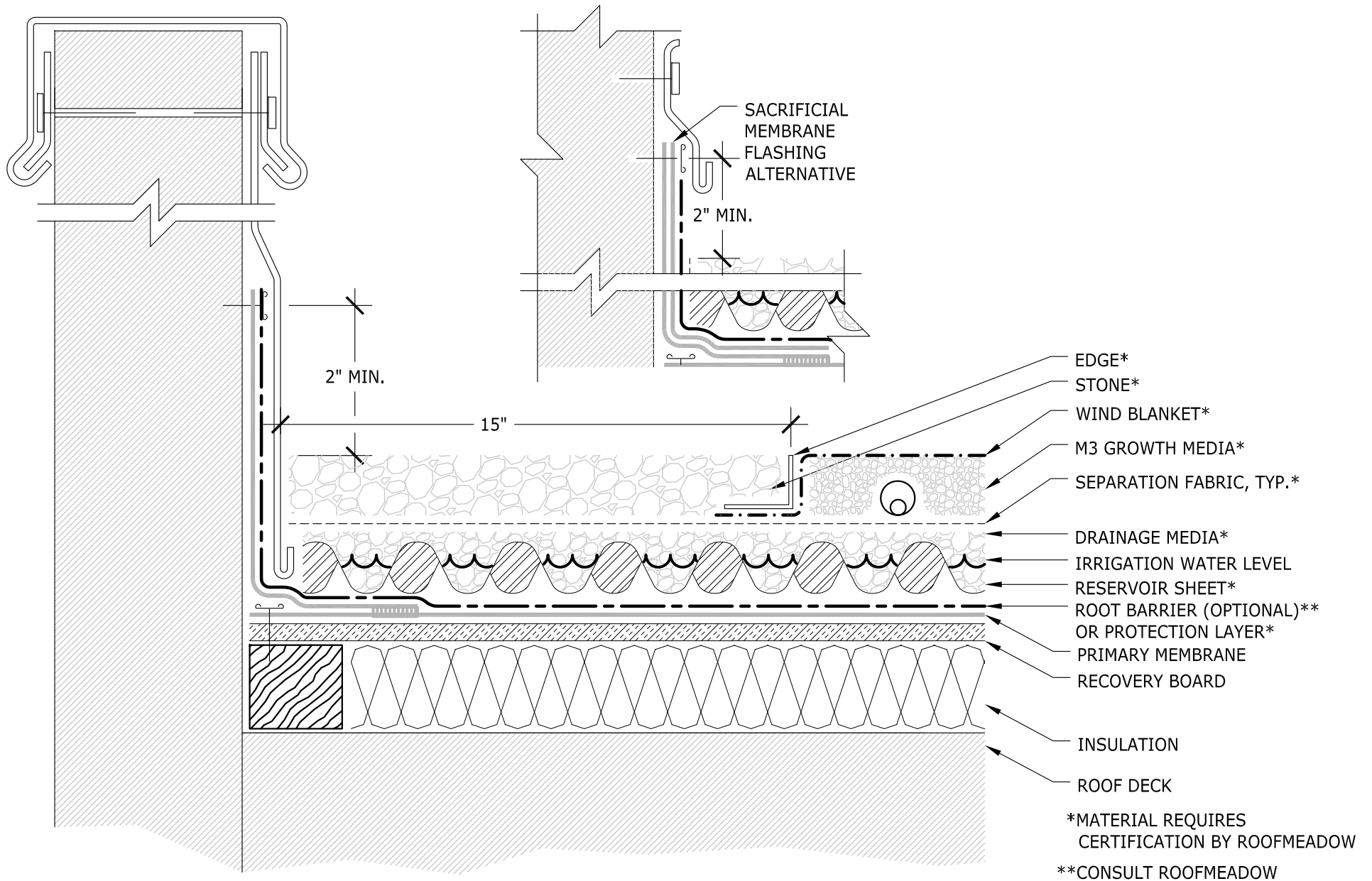
V - DUAL MEDIA WITH RESERVOIR SHEET CONVENTIONAL CONFIG. WITH INSULATION - AT PARAPET WITH STONE BORDER N.T.S.
