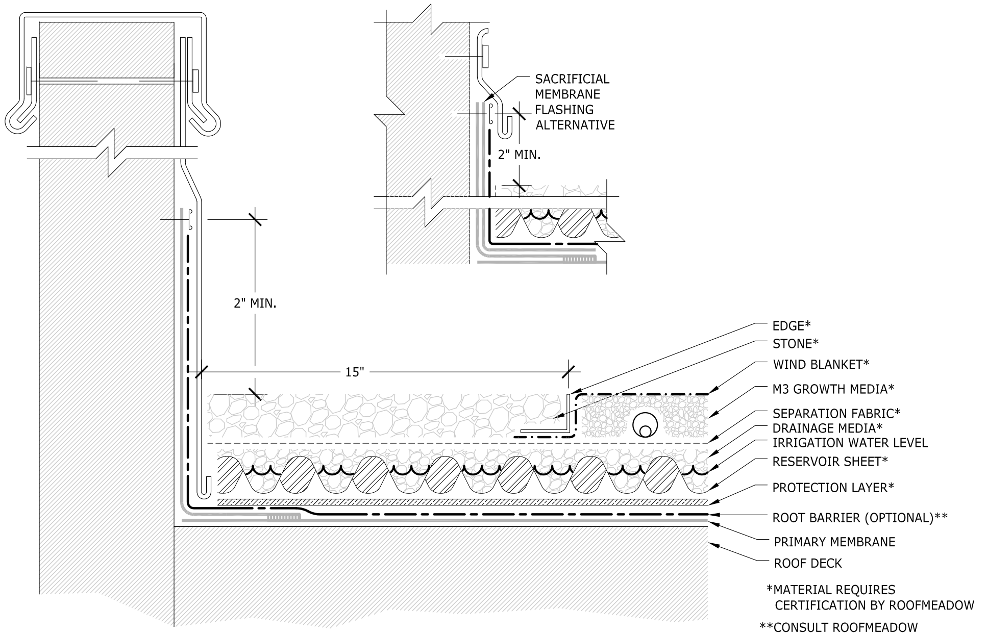
V - DUAL MEDIA WITH RESERVOIR SHEET CONVENTIONAL CONFIG. WITHOUT INSULATION - AT PARAPET
